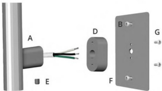
Figure 3: Bottom mount
