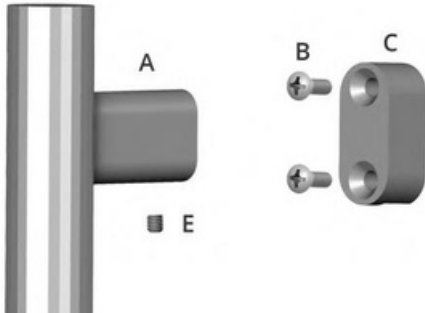
Figure 3: Bottom mount
