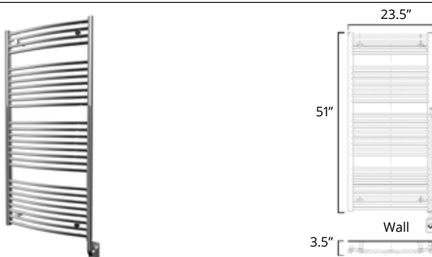
23.5" x 51" 300 Watts
