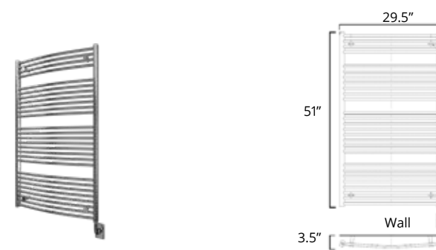
29.5" x 51" 300 Watts
