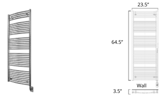
23.5" x 64.5" 450 Watts
