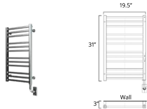
19.5" x 31" 150 Watts
