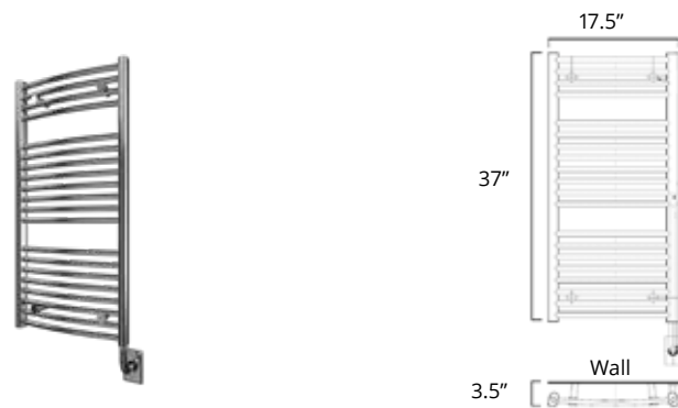
17.5" x 37" 300 Watts
